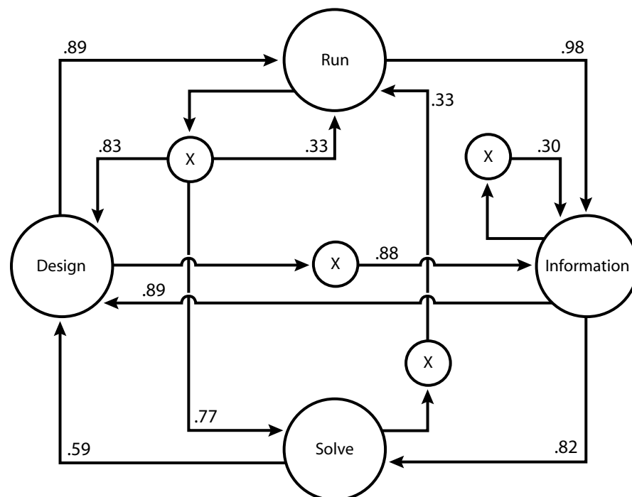
Figure 4. Lag 1 and lag 2 transitions (only values of Yule's Q greater than or equal to .30 are shown). All values are within a 95% confidence interval. X indicates any intervening event.
